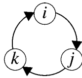
Figure 2. Quaternionic diagram.
