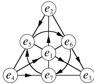
Figure 1. Fano plane representing the multiplication table for the octonions used throughout this paper.
